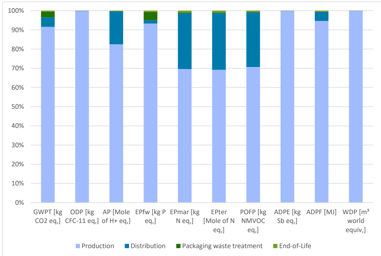
Figure 4: Breakdown of environmental impacts by life cycle stages (Average of Landfill and Recycling End-of-Life scenario/only Landfill scenario) See Table 5 and 6 for descriptions of environmental impact indicators).
